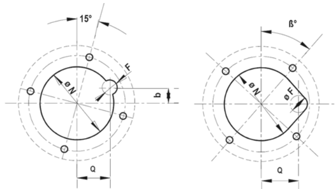
two assembly variants for size 15-80 up to 25-125
