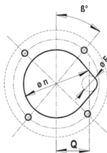
assembly opening size 32 -125
