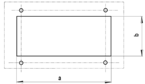
assembly opening size 32 -160 up to 80 - 250
